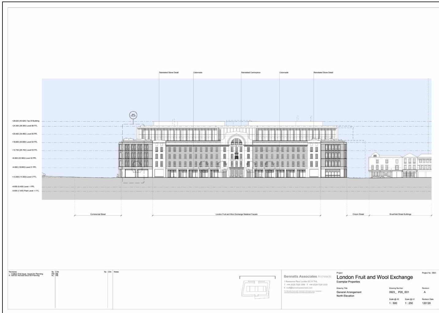
Proposed Brushfield Street elevation
