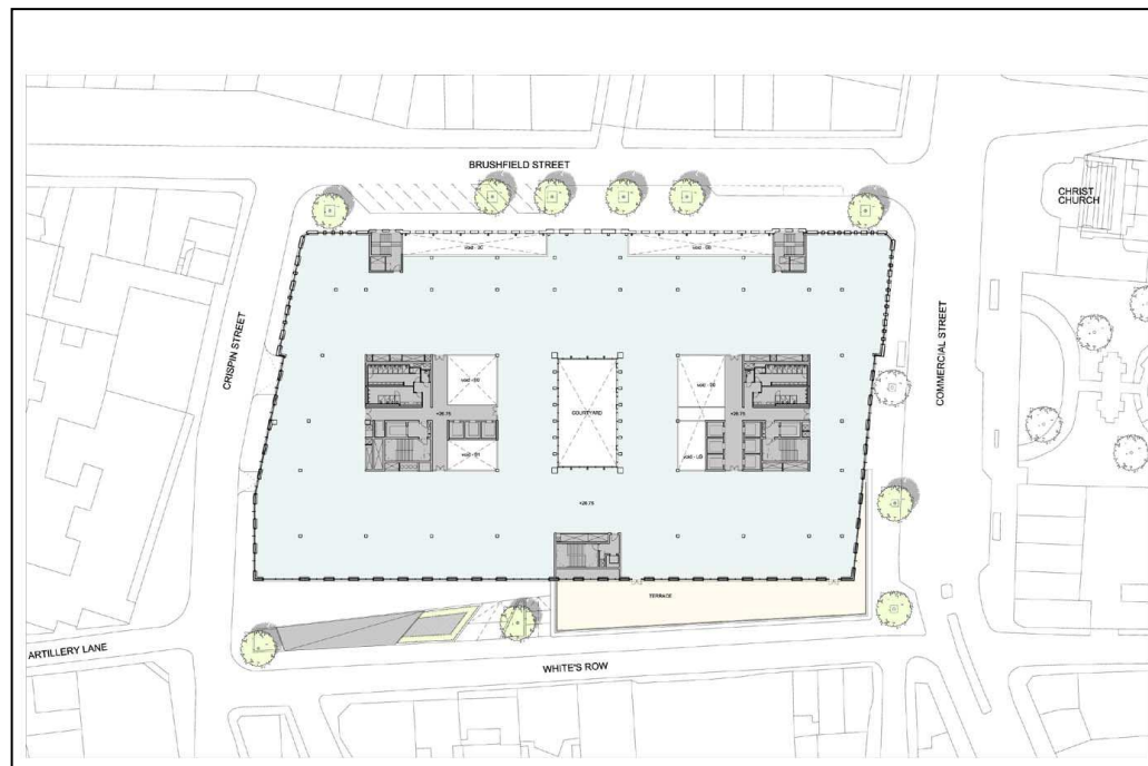
Typical upper floor layout (from TVAA)
